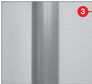
Standard natural clear anodised seamless drawn aluminium mast sections with \text{\O} 2\frac{1}{2} " (63,5 mm) base tube
